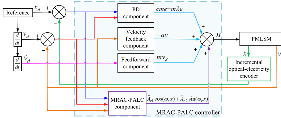
Fig. 3. Block diagram of the MRAC-PALC controller.
